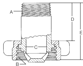
Style D For Vapor Equalizing
