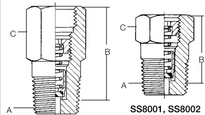
SS8001, SS8002 Series (.156 Orifice)
