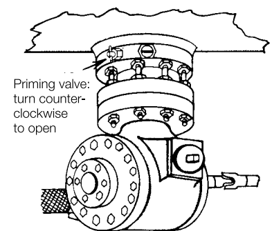
Figure 6. Priming Procedures
