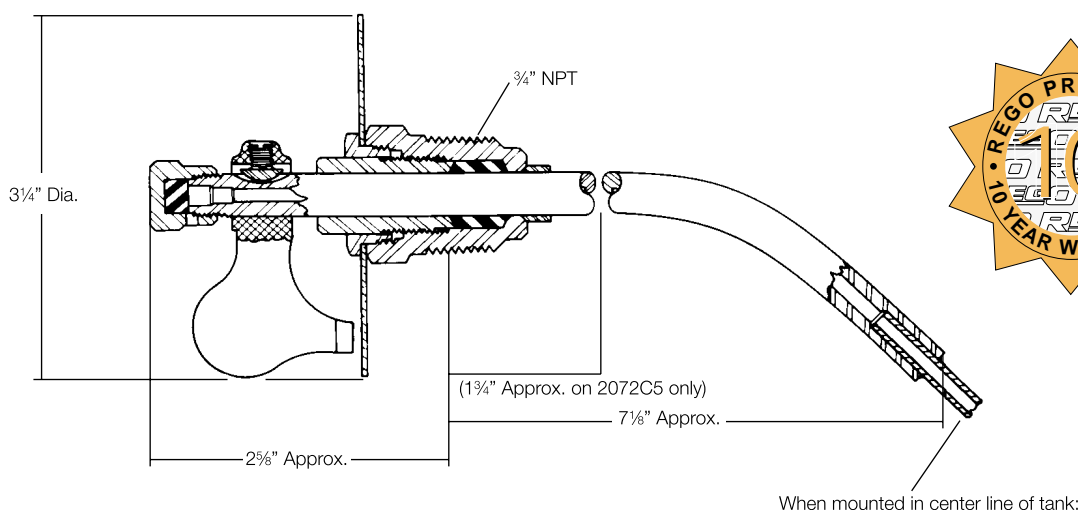
Side at Maximum Filling Level
