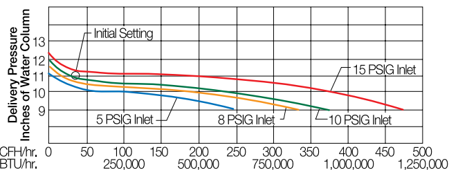
LV4403B Series
