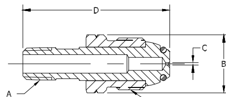
970S Soft Nose POL w/60 DMS Orifice
