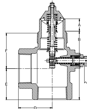
A3213D Series
