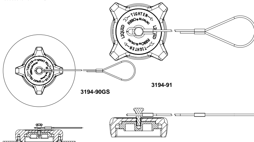
3194-91 Name plate
